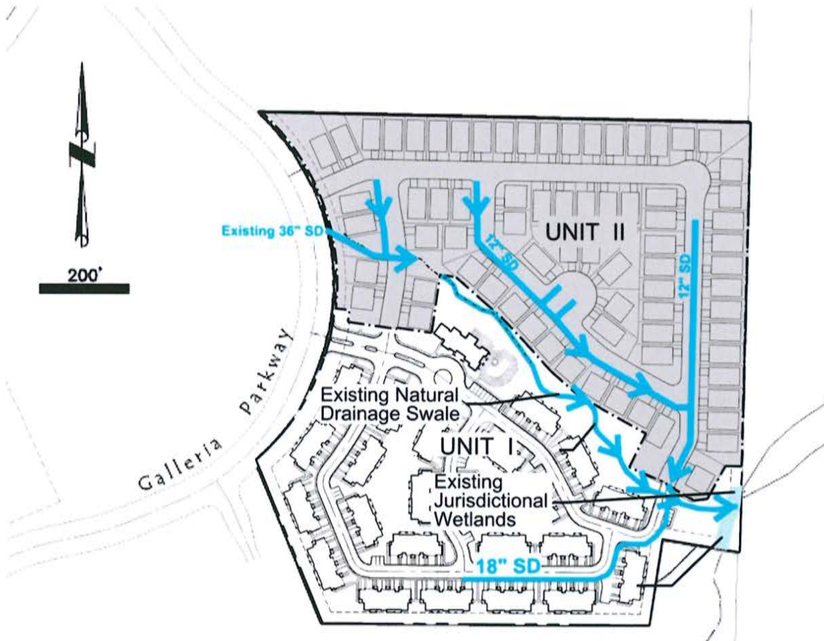
Figure 8 Phase I - Storm Drain Improvements
