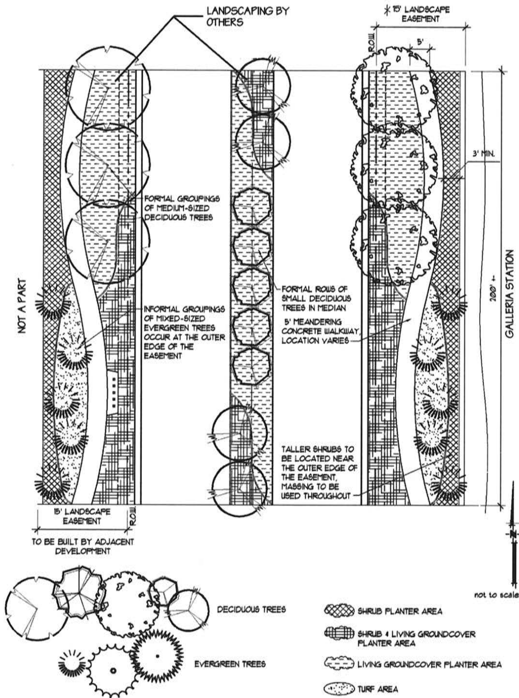
Figure 26 Galleria Parkway Streetscape
