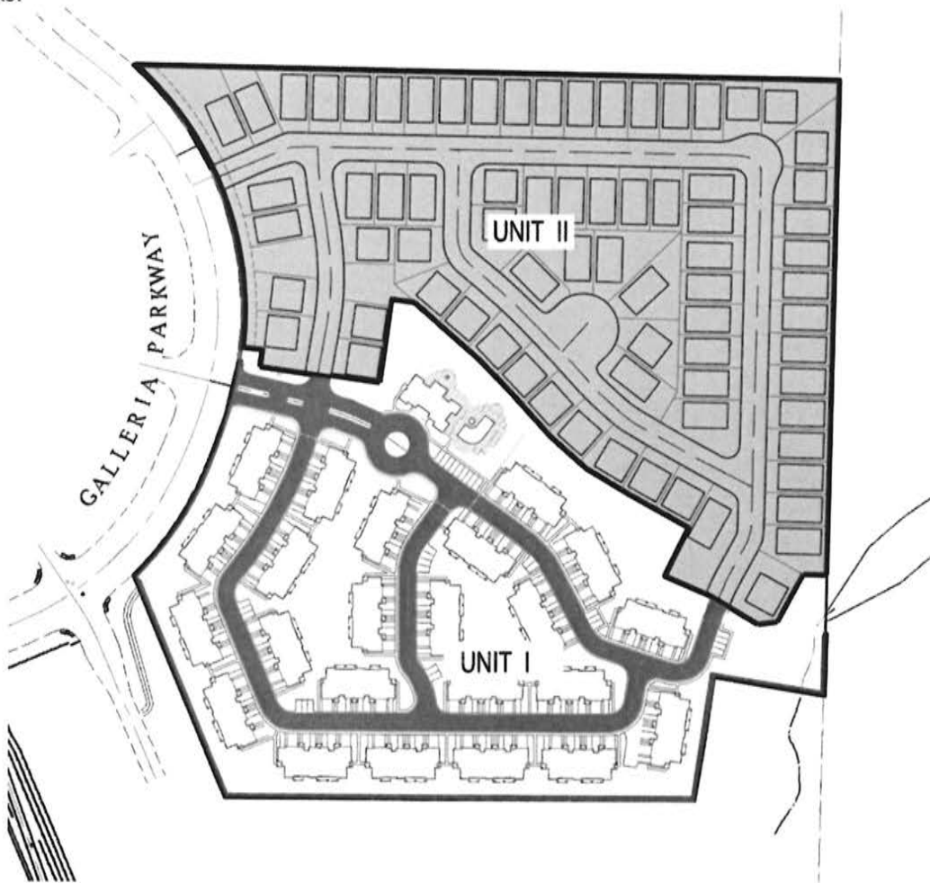
Figure 9 Roadways
