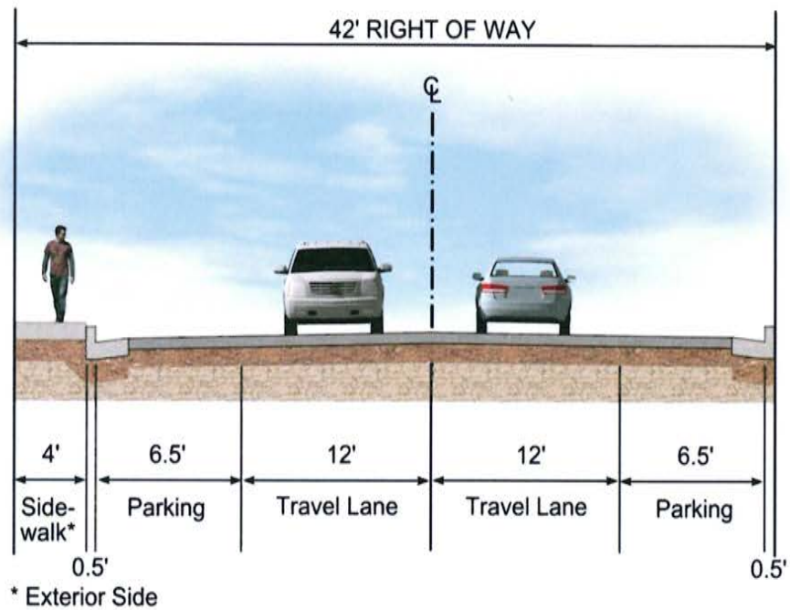
Figure 21 Unit II (Single-Family) Residential Street Section (Public)
