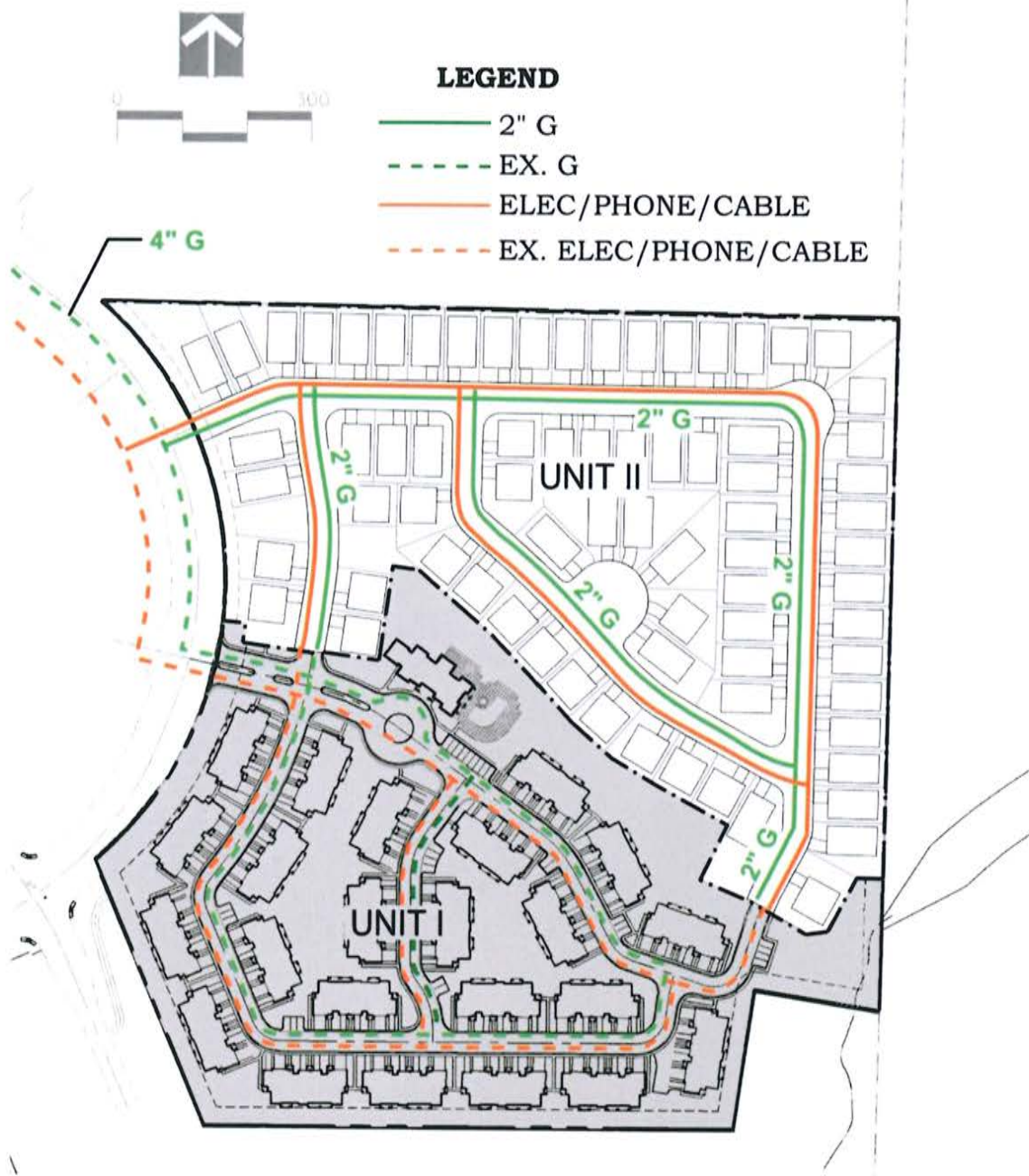
Figure 15 Phase II Utility Improvements
