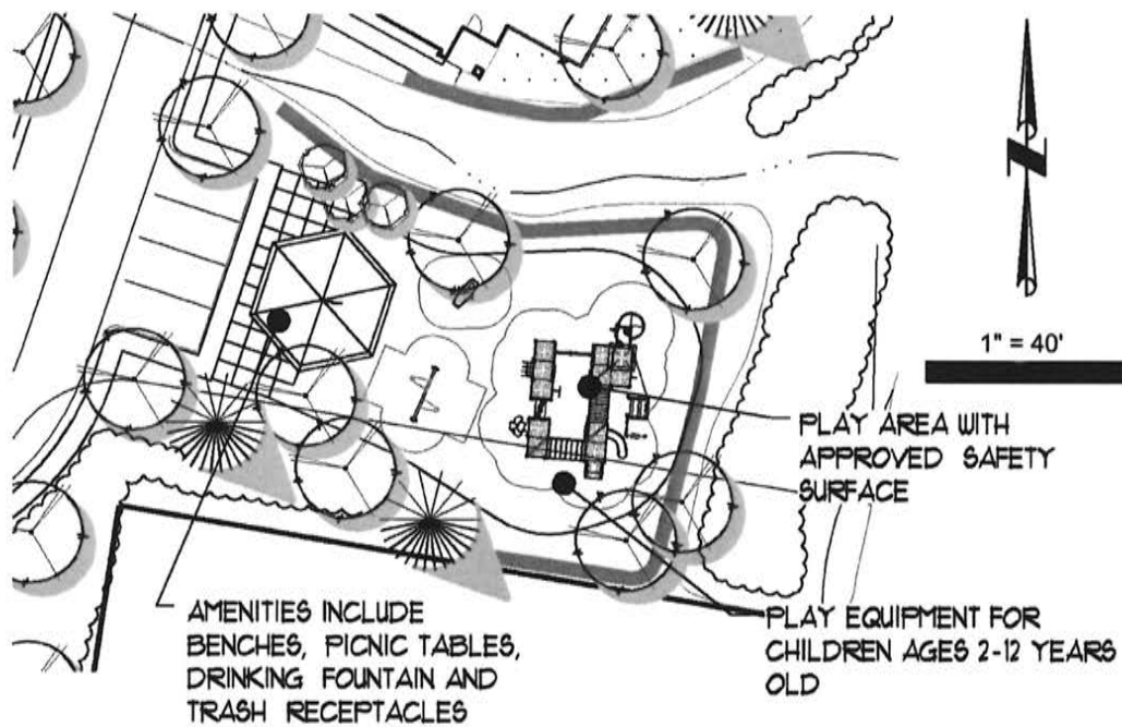
Figure 34 Tot Lot Recreation Area
