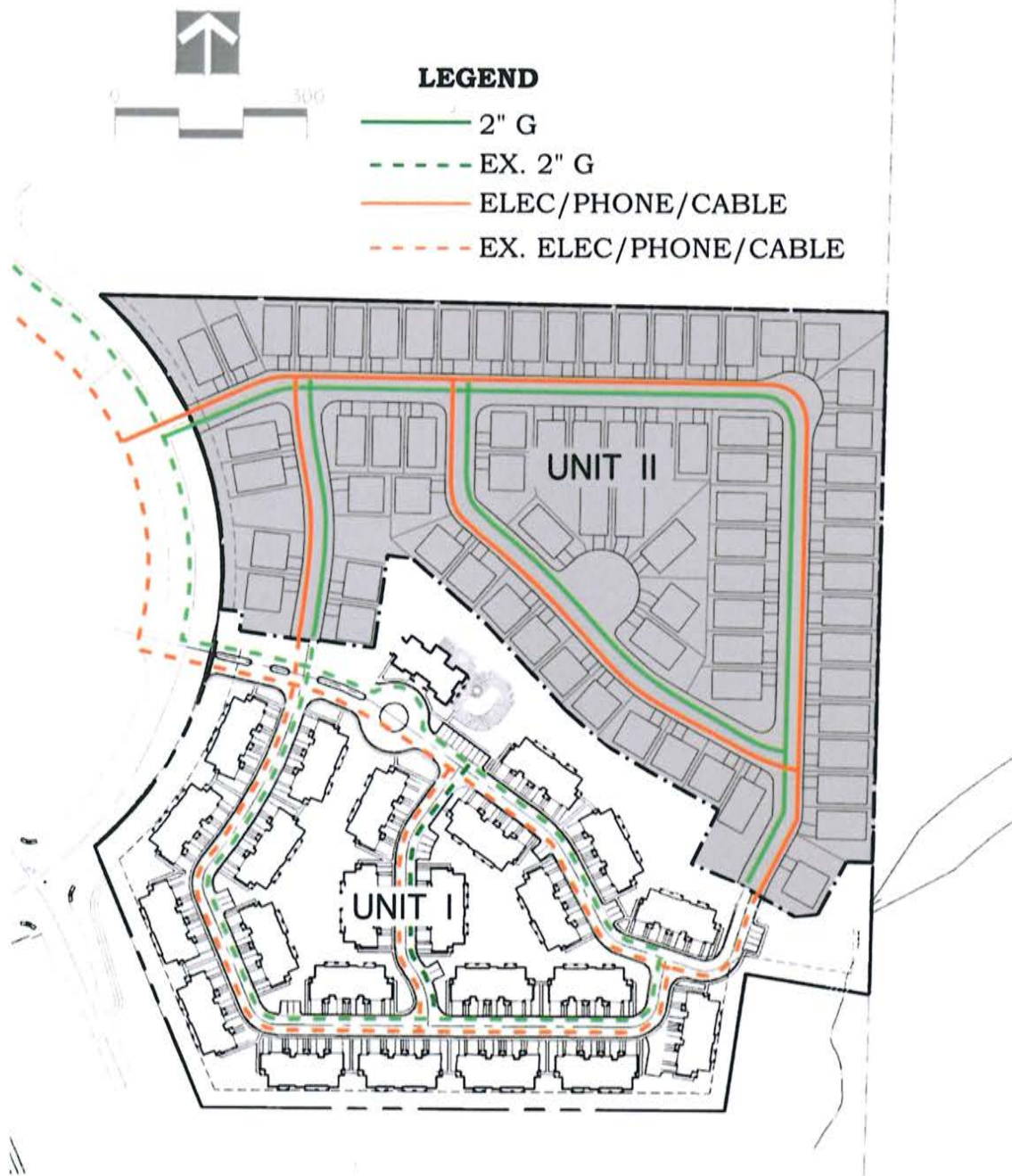
Figure 10 Phase I - Utility Improvements
