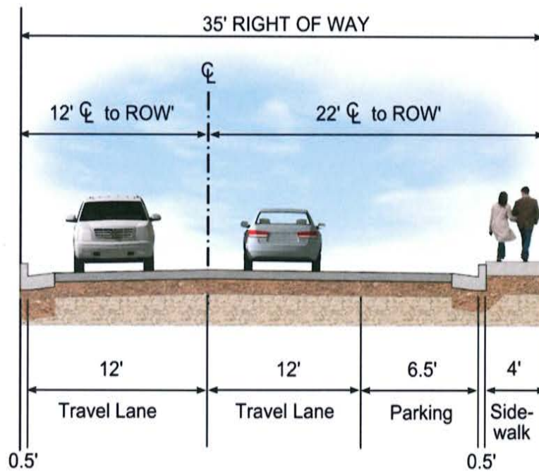
Figure 22 Unit II (Single-Family) Residential Street Section (Private)
