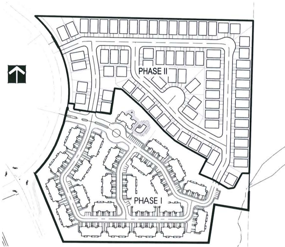
Figure 5 Galleria Station Phasing Plan
